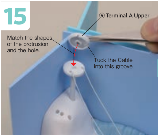
Assemble ⑨ Terminal A Upper on top of the upper Terminal.
