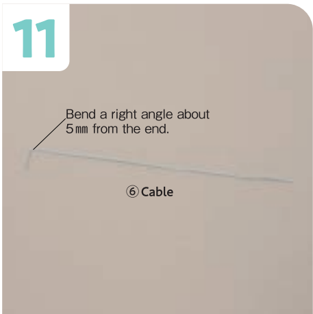
Bend a right angle about 5mm from the end of the ⑥ Cable as shown.
