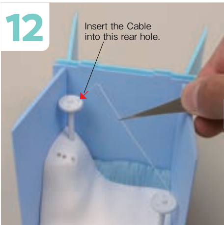
Insert the bent end of the ⑥ Cable into the rear hole of the upper Terminal.
