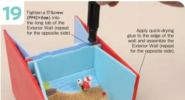
Assemble the Exterior Walls removed in step 1 back to the 【Sandcastles/Skiing】 scene box by tightening the ⑰ Screws (PM2×6mm) into the holes in the long tabs of the Exterior Walls, as we did before.
