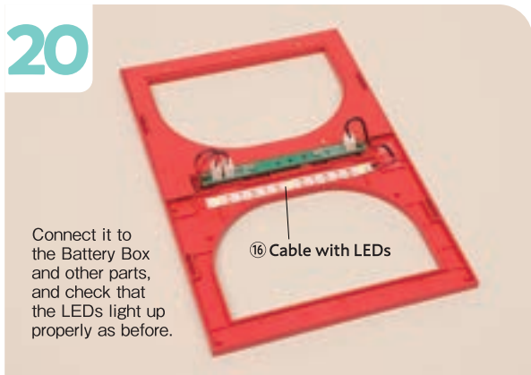
As before, affix the ⑯ Cable with LEDs to the Ceiling removed in step 1 in the position shown, and plug its connector into the socket on the Circuit Board.
